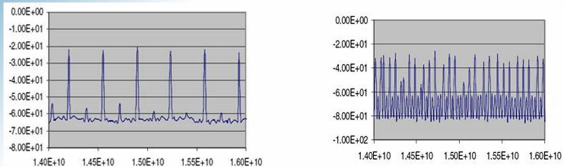
- Spectrum of a 44 Gbit/s PRBS Signal ( 2^7-1 ) (left) compared to a 40Gbit/s QPRBS ( 4 \times 10\text{Gbit/s PRBS } 2^7-1 ) (right) -
