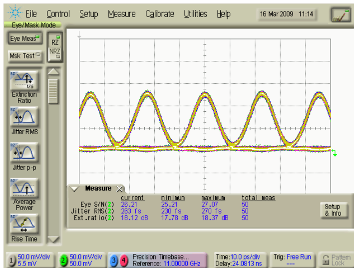
44 Gbps RZ optical output signal. S/N: 26, Jitter: 263 fs
