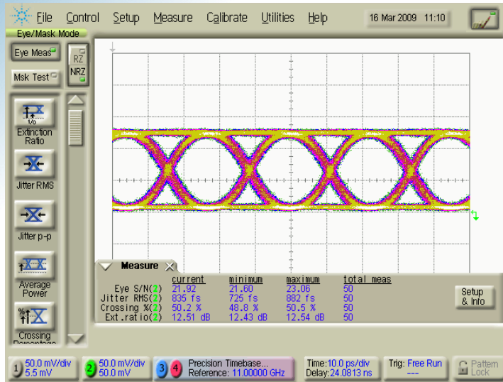
44 Gbps NRZ optical output signal. S/N: 21, Jitter: 835 fs
